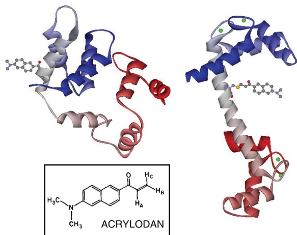
Fig. 3. Illustration of Ca 2+ -free ( Left ) and Ca 2+ -loaded ( Right ) CaM Acr . The crystal structures of Ca 2+ -free (PDB entry 1QX5) and Ca 2+ -loaded (PDB entry 1CLL) CaM were modified by using the program DS Viewer. ( Inset ) Structure of acrylodan.
