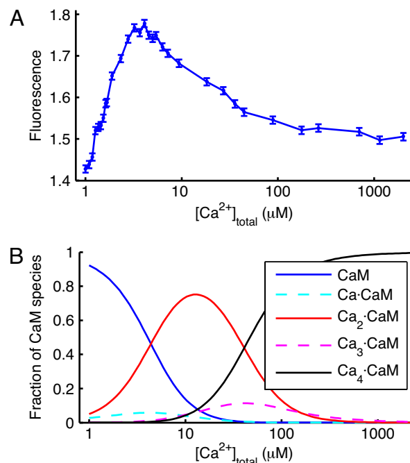
Fig. 4. Steady-state Ca 2+ binding to CaM. From the comparison of A and B , the fluorescence increase of CaM Acr upon addition of Ca 2+ is attributed to accumulation of Ca 2 ·CaM, and the fluorescence decrease is associated with population of Ca 4 ·CaM. ( A ) Fluorescence intensity of CaM Acr versus Ca 2+ concentration. CaM Acr was diluted to 200 nM in decalcified CaM dilution buffer and titrated with CaCl 2 . The sample was excited at 375 nm at room temperature ( \approx 20^\circ\text{C} ). The intensity was corrected for dilution of CaM Acr and normalized to the intensity of Ca 2+ -free CaM Acr , which was measured by adding 500 μM EGTA. ( B ) Fractions of CaM species binding different numbers of Ca 2+ ion versus total Ca 2+ concentration. The fractions were calculated from the macroscopic calcium binding constants of wtCaM.
