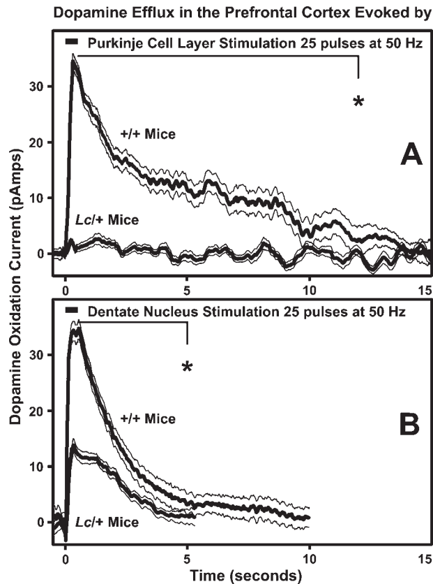
Fig. 2. Electrical stimulation (black bar, 25 pulses at 50 Hz, 200 \mu A) of the (A) Purkinje cell layer (PCL) or (B) dentate nucleus (DN) evokes a long lasting increase in prefrontal cortex DA efflux of wildtype (+/+) mice; an effect that is absent and markedly attenuated, respectively, in PCL and DN stimulated lurcher ( Lc/+ ) mice. In (A and B) the thick black lines and outer thin black lines are the mean \pm SEM, respectively ( n = 6 and 10 for PCL and DN stimulation in +/+, respectively, n = 10 and 10 for Lc/+ mice, respectively). * indicates significant difference from 0.5 to 12 s between +/+, and Lc/+ mice following PCL stimulation and significant difference from 0.5 to 5 s between +/+, and Lc/+ mice following DN stimulation.
