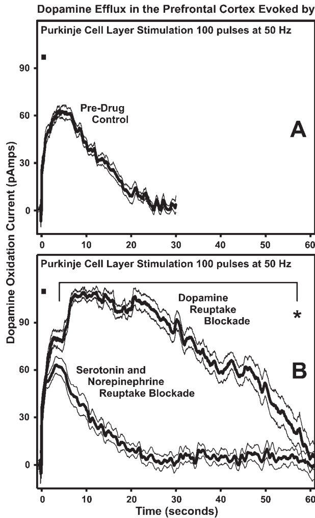
Fig. 3. Electrical stimulation (black bar, 100 pulses at 50 Hz, 200 \mu A) of the Purkinje cell layer evokes a long lasting increase in prefrontal cortex DA efflux of wildtype (+/+) mice (A); an effect that is significantly enhanced by selective blockade of DA reuptake with systemic administration of nomifensine, but unaffected by selective blockade of serotonin and norepinephrine reuptake with systemic administration of fluoxetine and desipramine, respectively (B). In (A and B) the thick black lines and outer thin black lines are the mean \pm SEM, respectively ( n = 6 +/+ mice for Pre-Drug Control and DA Reuptake Blockade groups and n = 9 +/+ mice for Serotonin and Norepinephrine Reuptake Blockade group). * indicates significant difference from 4 to 57 s between DA Reuptake Blockade group and Pre-Drug Control and Serotonin and Norepinephrine Reuptake Blockade groups.
