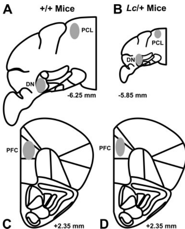
Fig. 1. Representative coronal sections of the wildtype ( +/+ ) and lurcher ( Lc/+ ) mouse cerebellum (A,B) and forebrain (C,D) (adapted from the mouse atlas of Franklin and Paxinos, 1997), with gray shaded areas illustrating placements of stimulating electrodes in the Purkinje cell layer (PCL) and dentate nucleus (DN) and electrochemical recording electrodes in the prefrontal cortex (PFC) (numbers correspond to mm from bregma). Note that the cerebellum of Lc/+ mice is approximately 50% the size of +/+ mice due to the 100% loss of Purkinje cells (Martin et al., 2003, 2006). Thus, based on preliminary histological analysis the stereotaxic coordinates for the PCL and DN were adjusted accordingly for these mice.
