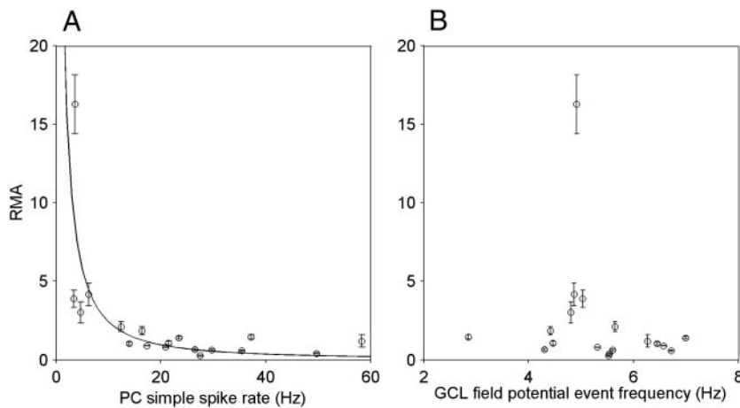
FIG. 5. Dependency of RMA on GCL field potential event frequency and PC spiking rate. A: PC spiking rates and RMA values are inversely related. This relationship can be demonstrated by the curve fit using a 2-parameter power function (—). B: The highest RMA values are centered within a narrow frequency between 4 and 6 Hz in GCL activity. Standard errors were calculated based on 20 RMA values determined by their background levels.
