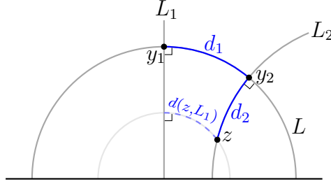
Figure 5.2: Illustration of Fact 5.2 (half-plane model of \mathbb{H}^2 )
