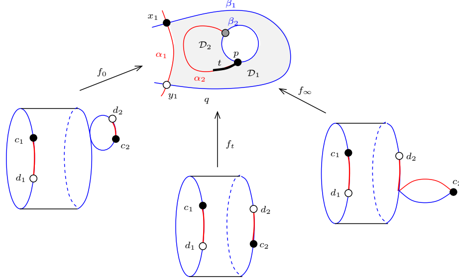
Figure 11.6. Varying the cut parameter in the proof of Proposition 11.4.7.
