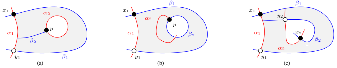
Figure 11.7. Domains for Exercise 11.4.8.
