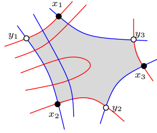
Figure 11.3. A non-elementary hexagon. The shaded domain from \mathbf{x} = \{x_1, x_2, x_3\} to \mathbf{y} = \{y_1, y_2, y_3\} is a hexagon.
