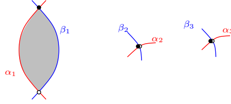
Figure 11.1. A bigon.
