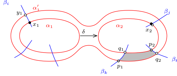
Figure 10.1. States after a handleslide. The state in \mathcal{H} locally represented by the intersection points \{x_1, x_2\} corresponds to a state in \mathcal{H}' represented by \{y_1, x_2\} . The state in \mathcal{H}' locally represented by \{p_1, p_2\} corresponds to another state in \mathcal{H}' locally represented by \{q_1, q_2\} . These latter two states can be connected by the shaded rectangle.
