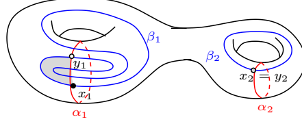
Figure 11.2. A non-elementary bigon. The shaded domain from \mathbf{x} = \{x_1, x_2\} to \mathbf{y} = \{y_1, y_2\} is a bigon.
