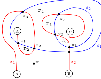
Figure 10.2. A genus 2 Heegaard diagram for S^3 .
