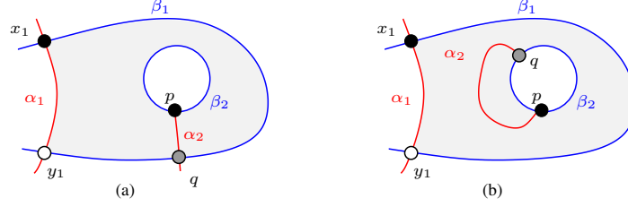
Figure 11.4. Domains homeomorphic to an annulus.
