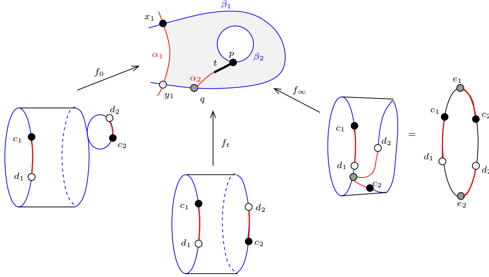
Figure 11.5. Varying the cut parameter in the proof of Proposition 11.4.5. The cut parameter t measures the length of the dark interval along \alpha_2 . For each t \in (0, \infty) , we have a cylinder and a uniformization map f_t . As t \rightarrow 0 , the cylinder degenerates a disk component; as t \rightarrow \infty , the cylinder degenerates to a disk with a double point on its boundary, i.e. identify e_1 and e_2 on the right-hand circle.
