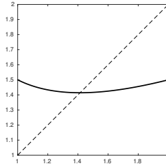
FIGURE 4. The function f(x) = \frac{1}{2} \left( x + \frac{2}{x} \right) (solid) and x \mapsto x (dashed).
