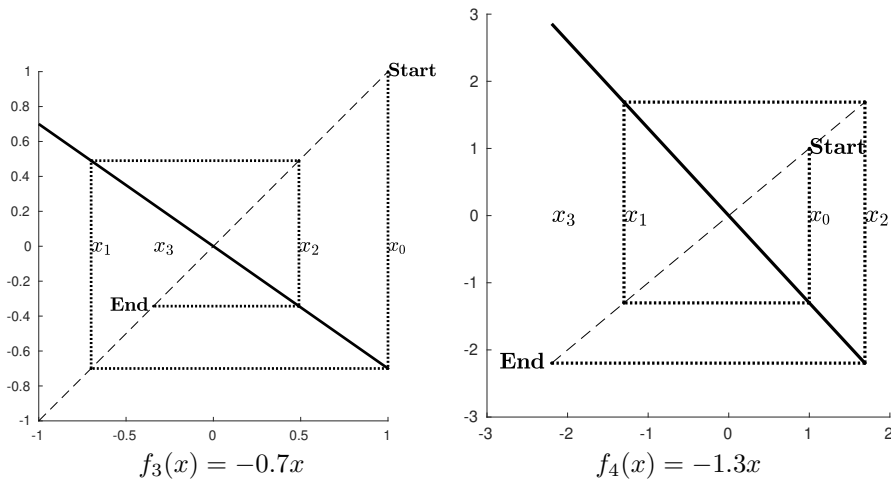
FIGURE 3. The iteration (5) for two linear functions with negative slope.
