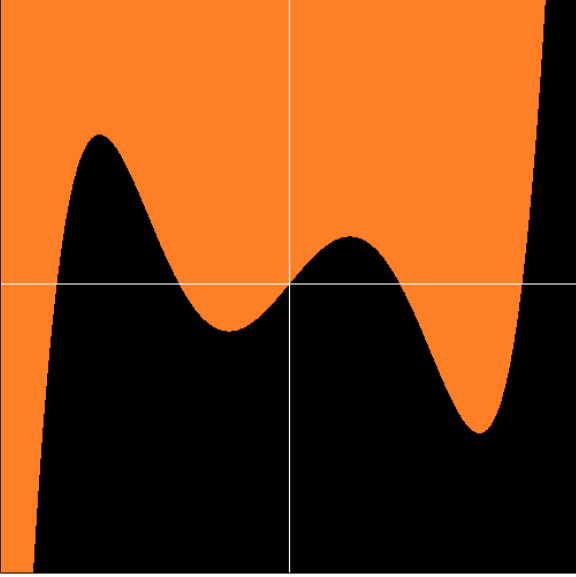
FIGURE 1. The partition of \mathbb{R}^2 used in [21] to show that K_G is smaller than Krivine’s bound; the shaded regions are separated by the graph y = c(x^5 - 10x^3 + 15x) .
