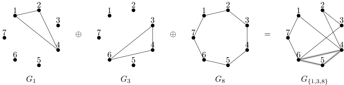
Figure 2: Graphs G_1, G_3, G_8 and their generated graph G_{\{1,3,8\}} in the proof of Proposition 17.
