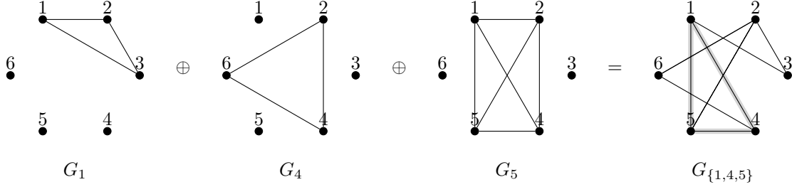
Figure 1: The graphs G_1, G_4, G_5 and their generated graph G_{\{1,4,5\}} in the proof of Proposition 16.
