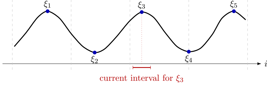
Figure 4: Schematic view of the polynomial construction. The items are consecutive points on the real line, and the polynomial has one turning point in each of \Theta(d) disjoint blocks. A comparison of two consecutive items near the midpoint of the current uncertainty interval determines on which side the corresponding turning point may lie, yielding a binary-search-type lower bound.
