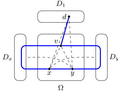
Figure 6: Proof of Lemma 4.2.
