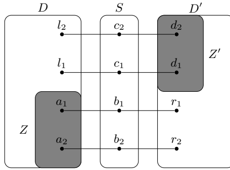
Figure 3: Definition of the set W .
