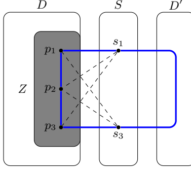
Figure 1: Proof of Lemma 3.2.
