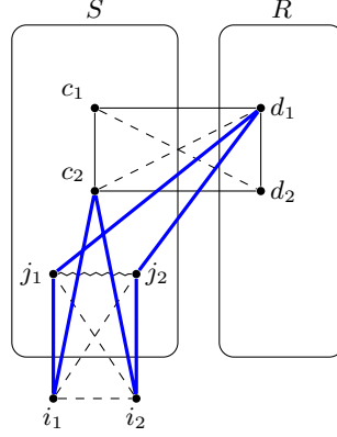
Figure 4: Proof of Lemma 3.6 in the case when c_2 is a common neighbor of i_1 and i_2 ; otherwise we use also l_2 to connect i_1 and i_2 . The edge j_1j_2 may be present.
