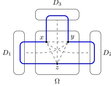
Figure 5: Proof of Lemma 4.1.
