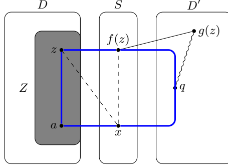
Figure 2: Proof of Lemma 3.4. The edge g(z)q may not be present.
