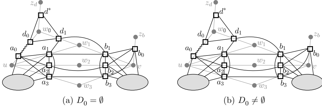
Figure 4: The construction of a larger strip-structure in (4.9). The gray vertices and edges represent the relevant submultigraph of H' . The black vertices and edges represent the relevant induced subtrigraph of T' . The gray ellipses represent the sets K_1 and K_2 . The ‘wiggly’ edge represents a semiedge. The black vertices are drawn on top of the gray edges to indicate to which strip each black vertex belongs.
