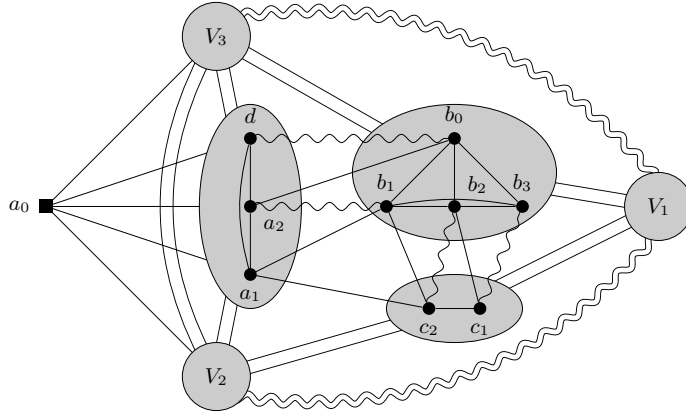
Figure 16: Schematic drawing of strips in \mathcal{Z}_{10} (Sporadic family of trigraphs of bounded size #3). V_2 is strongly complete to V_3 , and the adjacency between (V_1, V_2) and (V_1, V_3) is arbitrary. a_2, b_1 are semiadjacent; the pairs b_3, c_1 and b_0, d are either semiadjacent or strongly adjacent.
