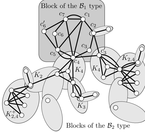
Figure 3: An example of the pattern multigraph H of an optimal representation (T, H, \eta) of an \mathcal{F} -free claw-free trigraph. The ellipses show the blocks of the multigraph. The pendant edges represent strips (J, Z) that satisfy 1 \leq |Z| \leq 2 . All other edges represent strips (J, Z) with |Z| = 2 .
