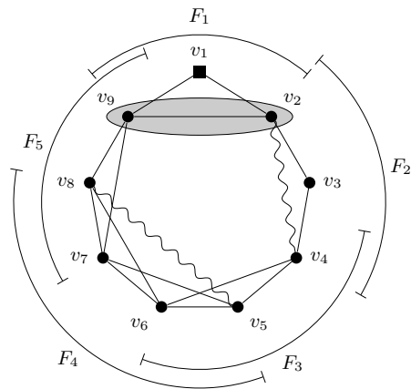
Figure 12: Example of a strip in \mathcal{Z}_6 (Long circular interval strips). v_1 is a simplicial vertex. The sets F_1, \dots, F_5 are the intervals.
