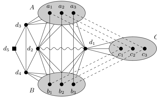
Figure 14: Schematic drawing of strips in \mathcal{Z}_8 (Augmented near antiprismatic strips). The pair d_1d_2 is either semiadjacent or strongly adjacent. There is essentially a matching between A and B , and there are complements of matchings between the sets A and C and between the sets B and C .
