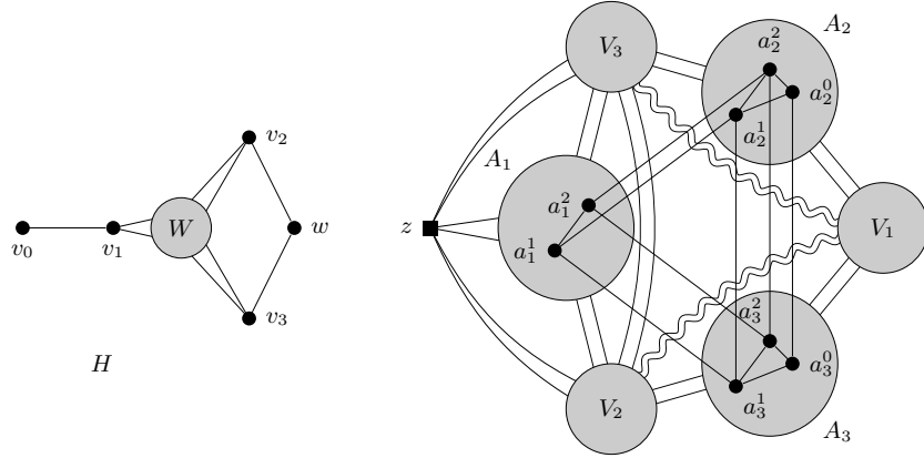
Figure 20: Schematic drawing of strips in \mathcal{Z}_{14} (Hex-expansions of line trigraphs). On the left: the graph H . The set W is a stable set. For i = 1, 2, 3 , the edges between v_i and W \cup \{w\} correspond to the vertices in A_i . The vertex w may be deleted. On the right: the corresponding hex-expansion of the line trigraph of H . V_2 is strongly complete to V_3 , and the adjacency between the pairs (V_1, V_2) and (V_1, V_3) is arbitrary. The vertices a_2^0, a_3^0 are either both present or absent (depending on whether w is present in H ).
