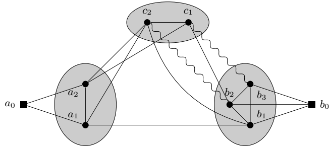
Figure 10: Schematic drawing of strips in \mathcal{Z}_4 (Sporadic family of trigraphs of bounded size #1). The pairs b_2, c_2 and b_3, c_1 are semiadjacent.
