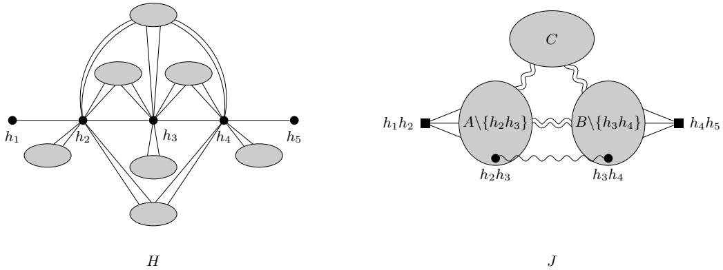
Figure 9: Schematic drawing of strips in \mathcal{Z}_3 . On the left: the graph H . On the right: the corresponding strip (J, Z) , which is almost a line trigraph of H , with the only exception that h_2h_3 and h_3h_4 are either semiajacent or strongly antiadjacent. The sets A, B, C satisfy A = \delta_H(h_2) , B = \delta_H(h_4) , C = \delta_H(h_3) \setminus \{h_2h_3, h_3h_4\} , where, for i \in \{2, 3, 4\} , \delta_H(h_i) is the set of edges in H that are incident with h_i .
