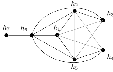
Figure 13: Schematic drawing of the graph H that underlies strips in \mathcal{Z}_7 (modifications of L(K_6) ). The graph H is the graph shown above, with possibly the edges of any subset of \{h_1h_3, h_2h_4, h_3h_5, h_2h_4, h_2h_5\} deleted (these edges correspond to the five edges ‘inside’ the 5-cycle h_1-h_2-h_3-h_4-h_5-h_1 ), and at most two of the edges \{h_6h_i \mid i = 1, 2, 3, 4, 5\} deleted. The trigraph J is essentially the line graph of H (regarded as a trigraph).
