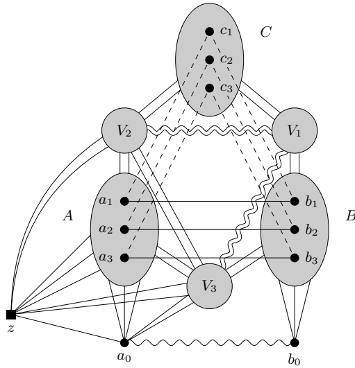
Figure 17: Schematic drawing of strips in \mathcal{Z}_{11} (Hex-expansions of near-antiprismatic trigraphs). There is essentially a matching between A and B , and there are complements of matchings between the sets A and C and between the sets B and C . V_2 is strongly complete to V_3 , and the adjacency between the pairs (V_1, V_2) and (V_1, V_3) is arbitrary. a_0, b_0 are either semiadjacent or strongly antiadjacent.
