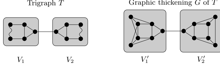
Figure 5: An example of a trigraph T (left) for which it is not possible to determine from the trigraph alone which leaf strip-block is the ordinary block given by (6.4). The graph on the right shows a \mathcal{F} -free graphic thickening of T .
