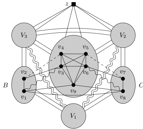
Figure 18: Schematic drawing of strips in \mathcal{Z}_{12} (Hex-expansions of of sporadic exception #2). V_1, V_2, V_3 are strong cliques. V_2 is strongly complete to V_3 , and the adjacency between the pairs (V_1, V_2) and (V_1, V_3) is arbitrary. The vertices v_3, v_4, v_5, v_6 may be deleted according to some rules.
