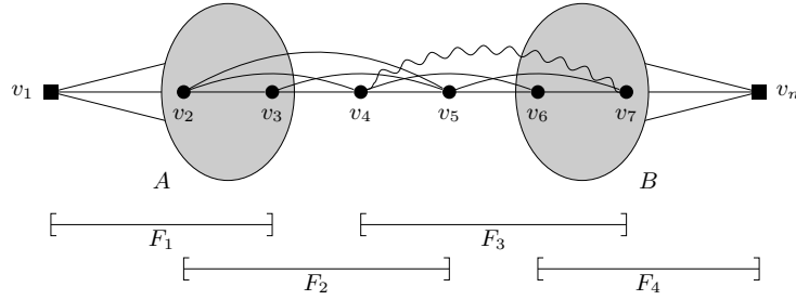
Figure 7: Schematic drawing of strips in \mathcal{Z}_1 (Linear interval strips). The sets A and B are strong cliques.
