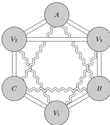
Figure 6: Schematic drawing of a hex-expansion. The sets A, B, C, V_1, V_2, V_3 are all strong cliques. The double lines indicate which sets are strongly complete to each other, the double curved line indicates which sets have arbitrary adjacencies between them.
