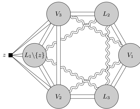
Figure 19: Schematic drawing of strips in \mathcal{Z}_{13} (Hex-expansions of circular interval trigraphs). L_1, L_2, L_3, V_1, V_2, V_3 are strong cliques. L_1 \cup L_2 \cup L_3 is a circular interval trigraph such that z is strongly anticomplete to L_2 \cup L_3 . V_2 is strongly complete to V_3 , and the adjacency between the pairs (V_1, V_2) and (V_1, V_3) is arbitrary.
