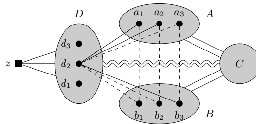
Figure 15: Schematic drawing of strips in \mathcal{Z}_9 (Special type of antiprismatic strips). There is essentially a complement of a matching between A and B . For every i and every d , d is strongly adjacent to one of a_i, b_i , and strongly antiadjacent to the other. The adjacency between C and D is arbitrary.
