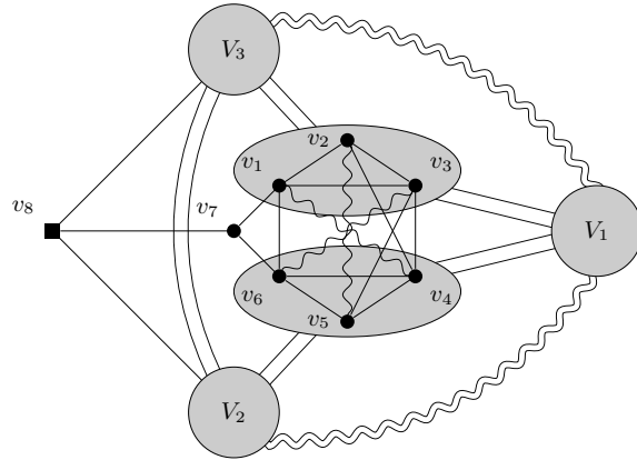
Figure 21: Schematic drawing of strips in \mathcal{Z}_{15} (Hex-expansions of sporadic exception #1). V_2 is strongly complete to V_3 , and the adjacency between (V_1, V_2) and (V_1, V_3) is arbitrary. The pairs v_1, v_4 and v_3, v_6 are semiadjacent, and the pair v_2, v_5 is either semiadjacent or strongly antiadjacent.
