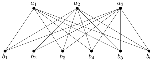
Figure 3: K(3, 6, 0) -subgraph.
