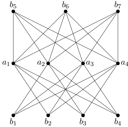
Figure 6: K(4, 7, 4) -subgraph.
