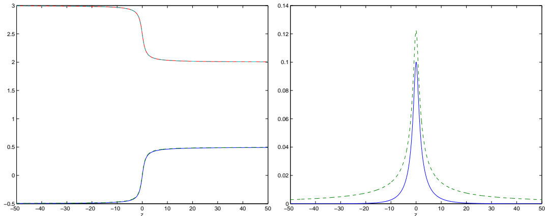
FIG. 2.1. The breakdown of the regular expansion. Left Panel: the leading order concentration (top / dashed) and potential (bottom / dashed) approximate well the corresponding numerical solutions (solid). Right Panel: The numerical net charge (solid) decays faster than the leading order Q_0 (2.8) (dashed). Inside the channel (near z = 0 ) the approximation seems to be reasonable, but it becomes poorer as we get further away from the channel into the bath.
