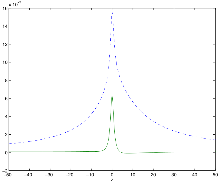
FIG. 4.1. Approximating the potential \phi : the approximation error of the leading order outer solution \phi_0^{OUT} - \phi (3.7) (dashed) and that of the uniform approximation \phi_{2,2}^{UNIFORM} - \phi (4.18) (solid).
