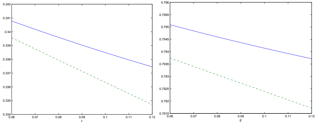
FIG. 4.2. Fluxes. Left Panel: The numerical diffusion flux (solid) and its first order approximation J_0^d + \varepsilon J_1^d (dashed). Right Panel: The numerical electric flux J^e (solid) and its first order approximation J_0^e + \varepsilon J_1^e (dashed).
