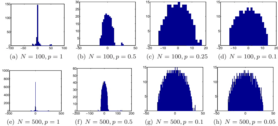
FIG. 5.1. Eigenvalue histograms for the matrix S for different values of N and p .
