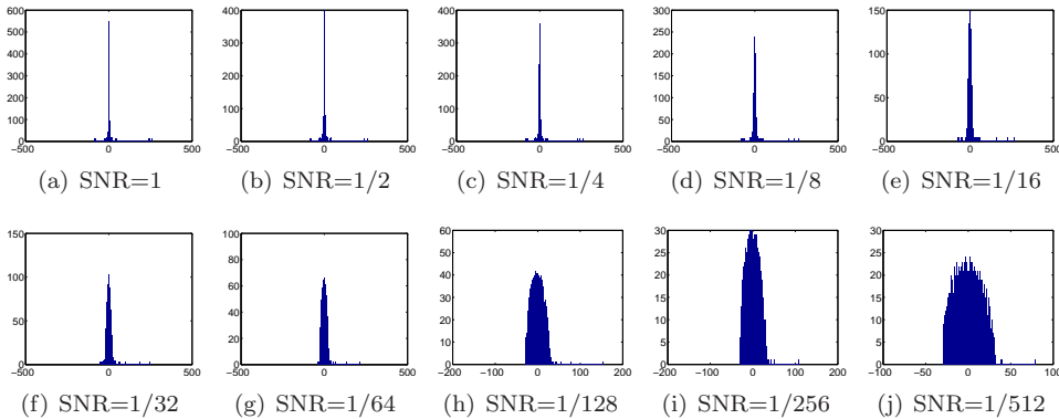
FIG. 5.4. Eigenvalue histograms of S for N = 500 and different levels of noise.
