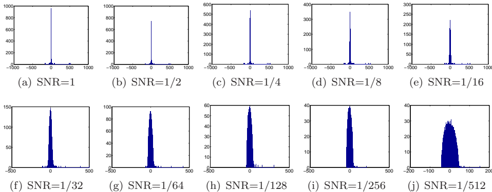
FIG. 5.5. Eigenvalue histograms of S for N = 1000 and different levels of noise.
