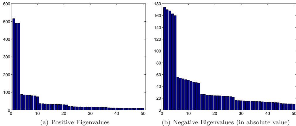
FIG. 6.1. Bar plot of the positive (left) and the absolute values of the negative (right) eigenvalues of S with N = 1000 and p = 1 . The numerical multiplicities 2l + 1 ( l = 1, 2, 3, \dots ) of the spherical harmonics are evident, with odd l values corresponding to positive eigenvalues, and even l values (except l = 0 ) corresponding to negative eigenvalues.
