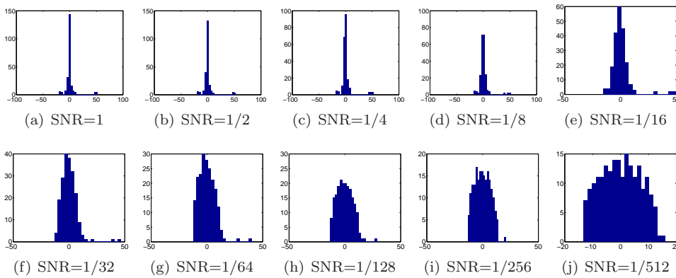
FIG. 5.3. Eigenvalue histograms of S for N = 100 and different levels of noise.
