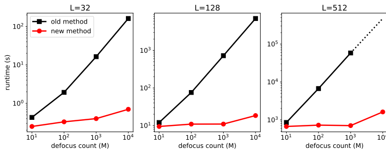
FIGURE 2. Timing comparison for covariance matrix estimation of 10000 images of size L \times L . The old method [4] timing for L = 512 and defocus count 10^4 is extrapolated due to time and memory constraints
