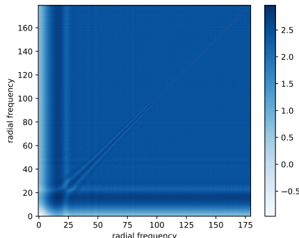
FIGURE 1. We visualize \log_{10} \left( \sum_{i=1}^N |\widehat{h}_i(|\xi|)|^2 |\widehat{h}_i(|\eta|)|^2 \right) for each pair of radial frequencies |\xi|, |\eta| for the experimental dataset EMPIAR-10028 [30] obtained from the Electron Microscopy Public Image Archive [12]. All values are greater than -1 in the log scale
