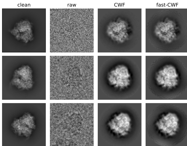
FIGURE 6. Denoised images (EMPIAR-10028). The method used N = 105247 images, from M = 1081 defocus groups, of size 360 \times 360 . The clean images are obtained by aligning 1000 clean projection images (from uniformly distributed viewing directions) with phase-flipped raw images
