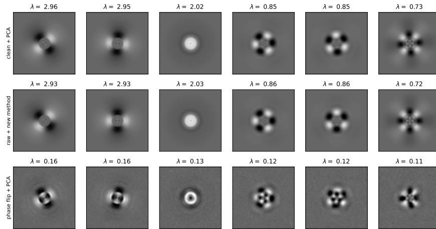
FIGURE 3. Top 6 eigenimages computed by traditional PCA on 10^6 clean images (top panel), our new method on 10^4 raw images (middle panel), and traditional PCA on 10^4 phase-flipped images (bottom panel). The signal-to-noise-ratio for the images for the new method and traditional PCA was 0.1
