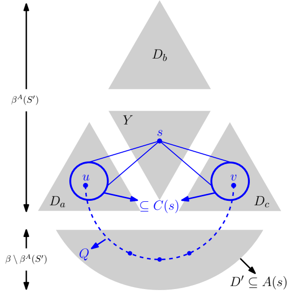
FIGURE 2. Proof of Theorem 4.11.
