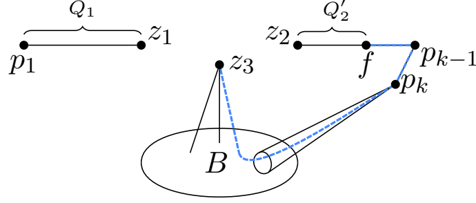
FIGURE 6. Visualization of Q_1, Q'_2 and Q'_3 (in blue).
