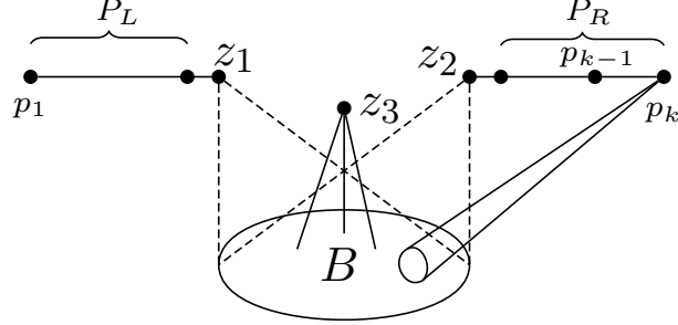
FIGURE 5. Visualization of G_h (here dashed lines represent non-edges).
