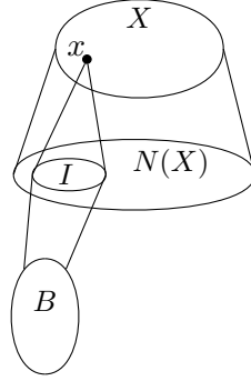
FIGURE 7. Drawing to keep in mind for the proof of Lemma 7.3.
