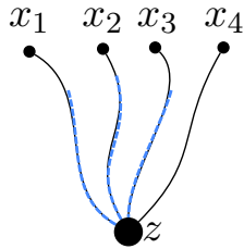
FIGURE 11. Visualization of the S_{t,t,t} obtained to prove (29).
