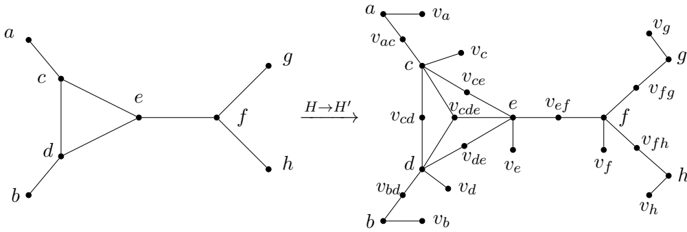
FIGURE 2. Example of H' given an H .
