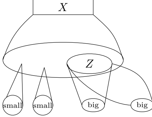
FIGURE 9. Visualization of G \setminus C in Theorem 7.6.
