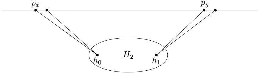
FIGURE 4. Visualization of h_0 and h_1 .
