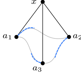
FIGURE 8. Visualization of the S_{t,t,t} obtained in the proof of (22).
