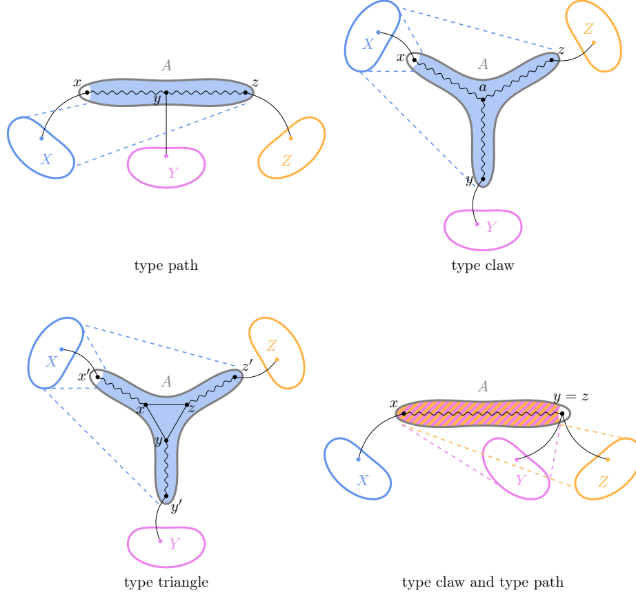
Figure 9: We illustrate the three types and a degenerate case in which type path and type claw overlap. For the three types we by way of example illustrate how X is not connected to anything in A but x . For the degenerate it is depicted that Y and Z are not connected to anything in A but the vertex y = z .
