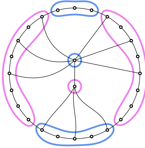
Figure 13: A K_{3,3} - e induced minor in an (even hole, triangle)-free graph
