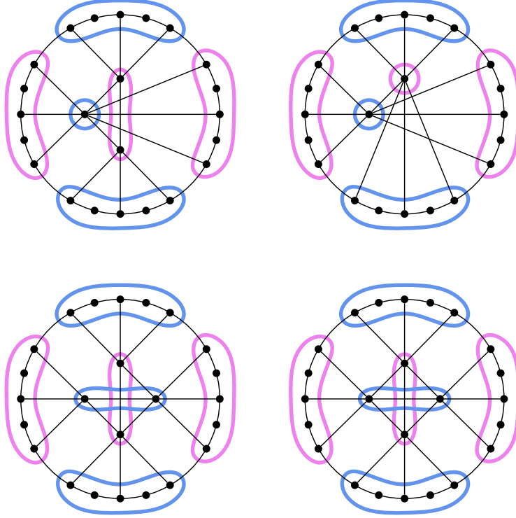
Figure 7: K_{3,3} as an induced minor in 3PC-free graphs
