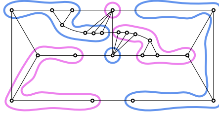
Figure 8: K_{3,3} as an induced minor in a (theta, prism)-free graph
