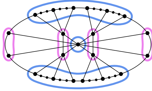
Figure 6: K_{3,4} as an induced minor while all 3PC's are prisms with a path of length zero
