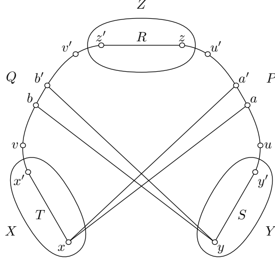
Figure 10: Paths P , Q , R , S and T in the proof of Lemma 5.1
