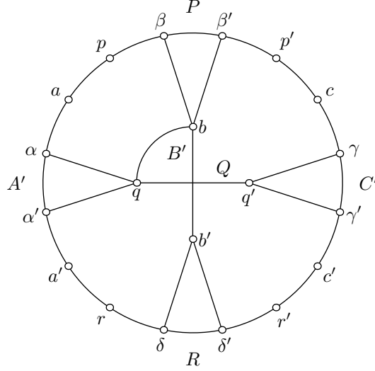
Figure 11: Paths A' , B' , C' , P , Q and R in the proof of Lemma 5.2
