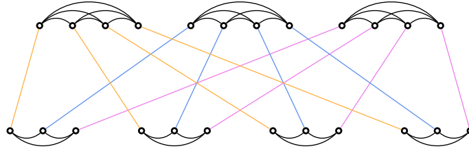
Figure 2: The line graph of the graph obtained by subdividing each edge of K_{3,4}
