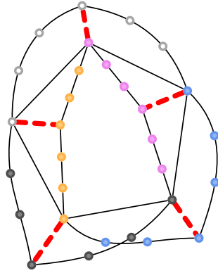
Figure 12: A K_5 minor in an (even hole, triangle)-free graph. To see even hole-freeness first note that no even hole can contain a fat red edge.
