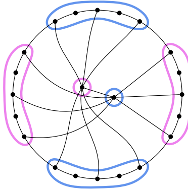
Figure 3: A (triangle, theta)-free graph containing K_{3,3} as an induced minor
