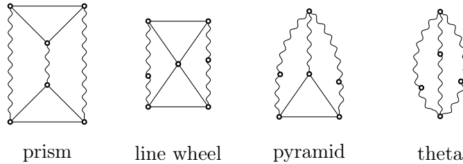
Figure 5: The different 3-path configurations
