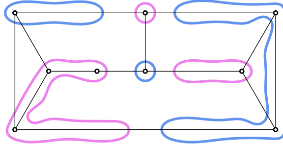
Figure 13: A K_{3,3} - e induced minor in an (even hole, triangle)-free graph
