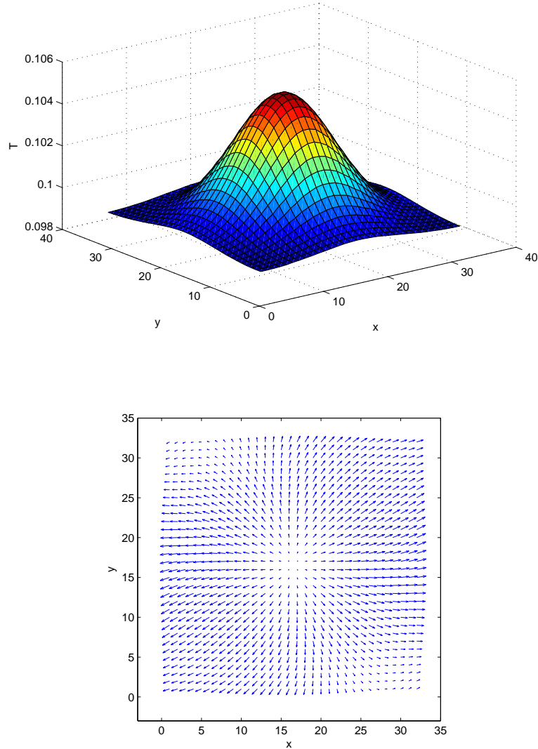
Fig. 7. Thermal expansion: temperature distribution (top) and the velocity field (bottom). The macro mesh consists of 36 \times 36 grid points. Each MD cell contains 36 \times 36 \times 3 \times 4 atoms, and the system is evolved for 10^4 time steps.
