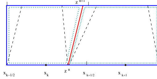
Fig. 9. A schematic demonstration of the defect tracking procedure. z^n represents the current interface location. The dotted line indicates the domain over which the PDEs (3) are integrated. The dashed line represents elastic waves generated from the Riemann problem, and the solid line in the middle indicates the interface.
