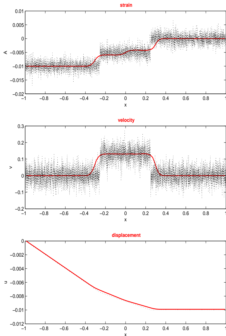
Fig. 6. Numerical test on shock formation and propagation. 200 macro-grid points are used and each local MD simulation consists of 40 \times 10 atoms and 10^4 steps of time integration. The solution is displayed after 40 steps of integration over macro time steps. Solid line: computed solution; dashed line: full atom simulation (one realization). Top: strain, middle: velocity, bottom: displacement.
