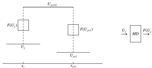
Fig. 1. A schematic illustration of the numerical procedure: starting from piece-wise constant solutions \{\mathbf{U}_j^n\} , one integrates (10) in time and in the cell [x_j, x_{j+1}] . To estimate \mathbf{F} at x_j , we perform a MD simulation using \mathbf{U}_j^n as constraints. This is indicated in the picture by small boxes.
