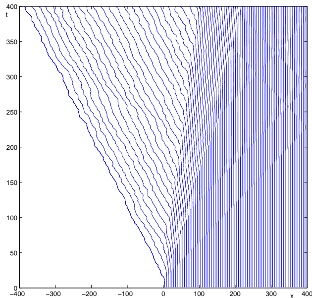
Fig. 12. Particle trajectory of the 1-d chain simulation: initially all the particles are at rest, with local strain in the first well. Then we start pulling the left end with a constant speed v = -1.0 . A phase boundary and a sound wave are clearly observed.
