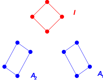
Fig. 16. Arrangement of the atoms in the cubic and tetragonal structure on the \{001\} plane: the deformation of the cubic phase is taken to be identity, while the two martensitic variants have deformation gradient given by (23).
