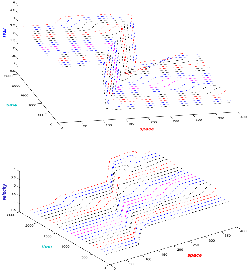
Fig. 14. Snapshots from the simulation: a phase boundary is present initially and the right end is pulled with constant speed. The shock wave and the phase boundary then collide. After the collision, a reflected and a transmitted wave are generated.
