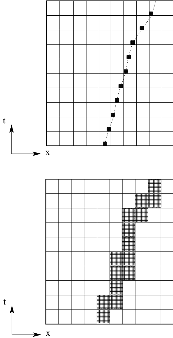
Fig. 8. Schematic of the adaptive modeling refinement. The top figure shows the case where T_r \ll T_d . The MD simulations are reinitialized at every macro time step. The dashed lines represents the interface. The bottom figure shows the other case where T_r and T_d are comparable. Here one has to keep track the local defect structure for all time.
